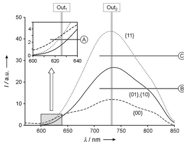
Figure 5. Luminescence spectrum ( \text{CH}_3\text{CN} , 293 K, excitation at an isosbestic point at 493 nm) of a newly prepared solution containing 2.4 \times 10^{-5} M Ru-H 2 4+ and 4.8 \times 10^{-5} M SP (dotted line). The dashed line represents the spectrum after 5 d in the dark at 293 K, at which point the solution contains mostly Ru 2+ and ME-H + . Upon partial irradiation (15 min) of the thermally equilibrated solution at 400 nm, the spectrum represented by the solid line is obtained, which is in agreement with the formation of the Ru-H 3 + species. Further exhaustive irradiation regenerates the initial spectrum (dotted line). The inset shows a magnification of the 600–640 nm region. Input strings, output wavelengths ( Out 1 , Out 2 ), and threshold values ( A , B , and C ) relevant for the binary logic operations are indicated.
