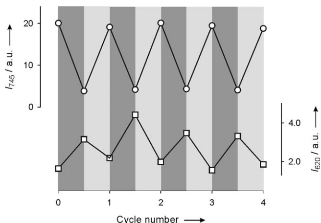
Figure 2. Emission-intensity values at 745 nm ( \circ , left scale) and 620 nm ( \square , right scale) upon several equilibration–irradiation cycles performed on a solution containing a 1:1 mixture of 1.6 \times 10^{-5} \text{ M} \text{Ru-H}^{3+} and \text{SP} . Conditions: thermal equilibration (dark gray areas), 10 h in the dark at 318 K; light irradiation (light gray areas), 90 min at 400 nm.
