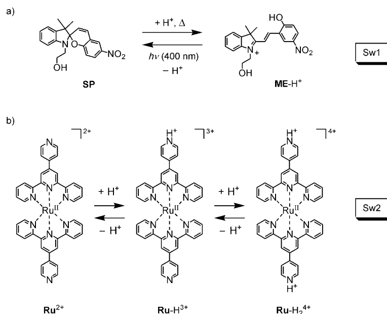
Scheme 1. Structure of the two molecular switches. a) Sw1: The acid- and light-controlled equilibrium between the spiropyran SP and the protonated merocyanine ME-H + . b) Sw2: The acid–base-driven interconversion between the three protonation states of metal complex Ru 2+ .
