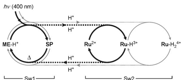
Figure 3. Coupled operation of the two-state switch Sw1 and three-state switch Sw2 by means of light-induced proton exchange. Irradiation of ME-H + such that one equivalent of protons is transferred to the metal complex generates the Ru-H 3 + state (thick lines). Further irradiation of ME-H + can cause the transfer of another equivalent of protons to the metal complex, thereby generating the Ru-H 2 4+ state (thin lines). Subsequent thermal equilibration in the dark regenerates the initial state by reverse proton exchange.
