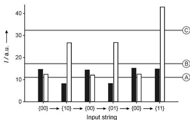
Figure 6. Response of the device to different input strings and cycling. Shaded and white bars represent the experimental luminescence intensities at 626 nm ( \text{Out}_1 ) and 732 nm ( \text{Out}_2 ), respectively. The intensity values at 626 nm have been multiplied by five for the sake of clarity. Marks A, B, and C represent the threshold values for the XNOR, OR, and AND operations, respectively (see Table 1). The experimental conditions are those described for Figure 5. Input conditions: {00}, 10 h at 318 K; {10} and {01}, irradiation at 400 nm for 15 minutes; {11}, exhaustive irradiation at 400 nm.
