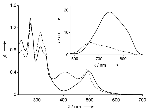
Figure 1. Absorption and (inset) luminescence spectra ( \text{CH}_3\text{CN} , 293 K) of a newly prepared solution containing a 1:1 mixture of 1.6 \times 10^{-5} \text{ M} \text{Ru-H}^{3+} and \text{SP} (solid line). The dashed lines represent the spectra after 5 d in the dark at 293 K, at which point the solution contains \text{Ru}^{2+} and \text{ME-H}^+ . Upon exhaustive irradiation of the thermally equilibrated solution at 400 nm, the spectra represented by the solid lines are restored. For the luminescence spectra, excitation was performed at an isosbestic point at 493 nm.
