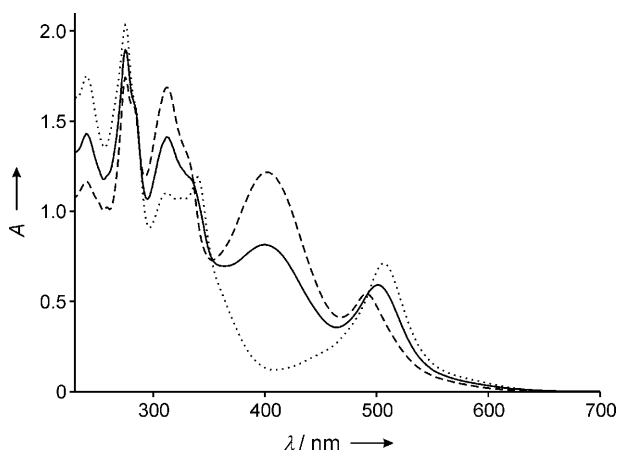
Figure 4. Absorption spectrum ( \text{CH}_3\text{CN} , 293 K) of a newly prepared solution containing 2.4 \times 10^{-5} M Ru-H 2 4+ and 4.8 \times 10^{-5} mol L -1 SP (dotted line). The dashed line represents the spectrum after 5 d in the dark at 293 K, at which point the solution contains mostly Ru 2+ and ME-H + . Upon partial irradiation (15 min) of the thermally equilibrated solution at 400 nm, the spectrum represented by the solid line is obtained, which indicates the formation of the Ru-H 3 + species. Further exhaustive irradiation regenerates the initial spectrum (dotted line).
